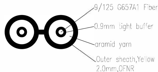
Ø2.0mm OFNR cable section
