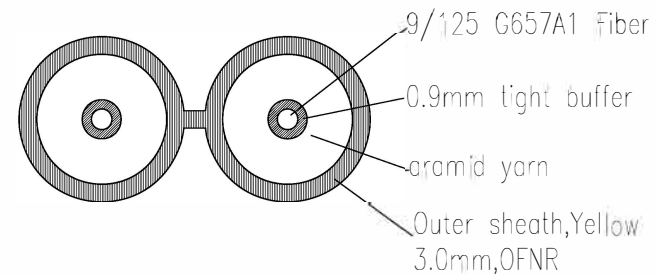
∅3.0mm OFNR cable section
